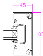
DETAIL G - G
