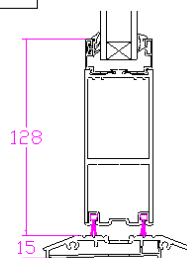
DETAIL D - D
