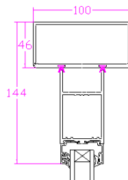
DETAIL A - A
