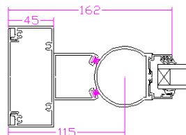
DETAIL B - B
