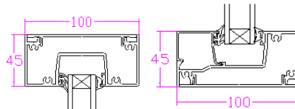
DETAIL H - H
